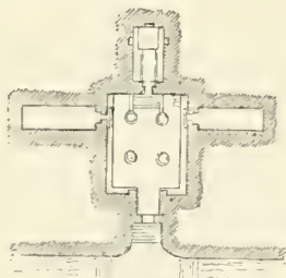
FIG. 234.—The speos at Addeh; plan from Hureau.
