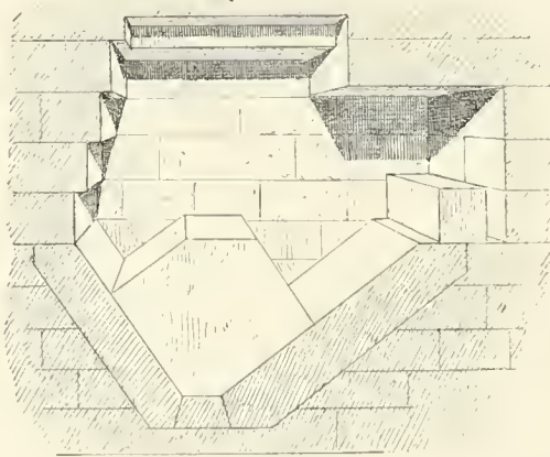
FIG. 151.—Portcullis closed.
