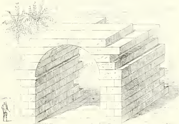
FIG. 76.—Off-set semicircular arch.
