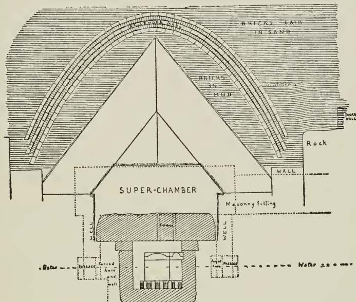
FIG. 92. SECTION OF THE BURIAL CHAMBER IN THE PYRAMID OF HAWARA. (After Petrie.)
