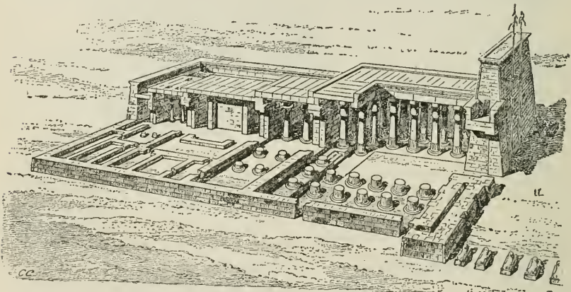
FIG. 126. PERSPECTIVE AND SECTION OF A TYPICAL PYLON TEMPLE OF THE EMPIRE.
