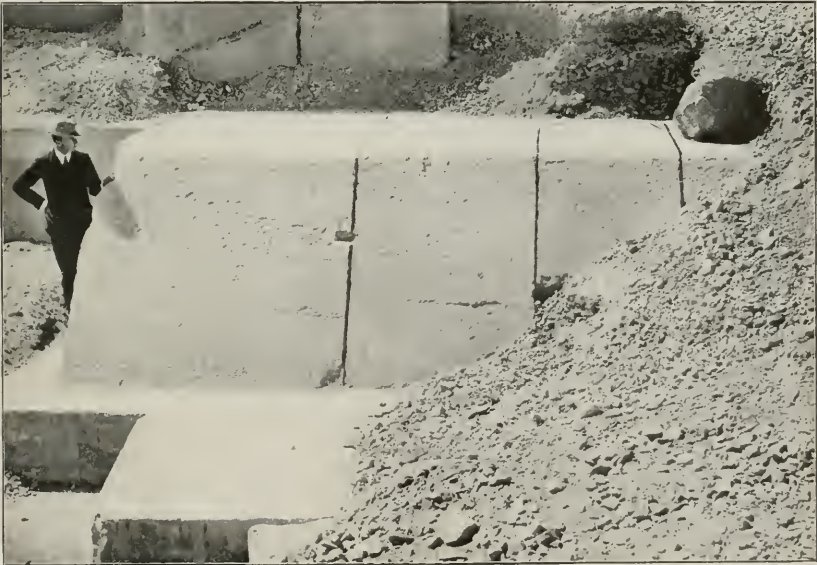
FIG. 66 —CASING BLOCKS AT THE BASE OF THE GREAT PYRAMID. JOINTS OTHERWISE UNDISCERNIBLE INDICATED BY CHARCOAL LINES.
