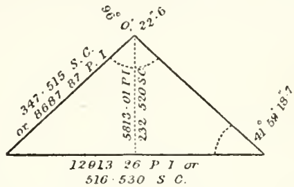
DIAGONAL VERTICAL SECTION OF GREAT PYRAMID.
