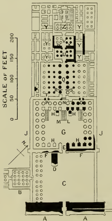
PLAN OF THE RAMESSEUM
